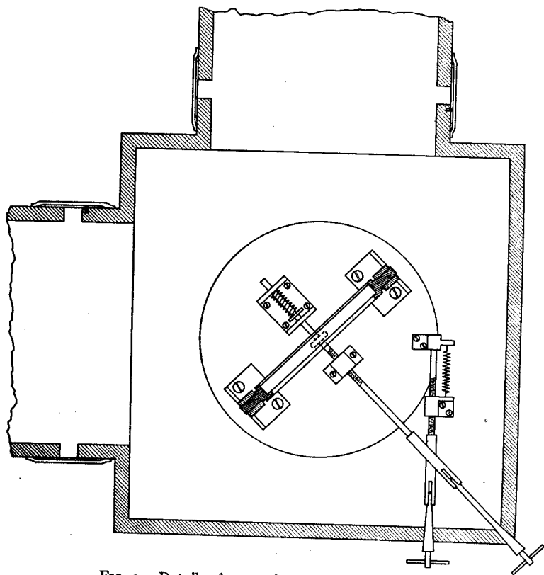
FIG. 2.—Details of corner box and mirror mounting
